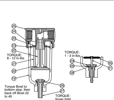
Figure 2: Particulate Filter
